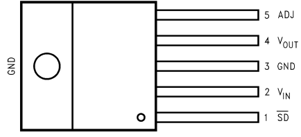
Top View TO220-5 Package Bent, Staggered Leads
